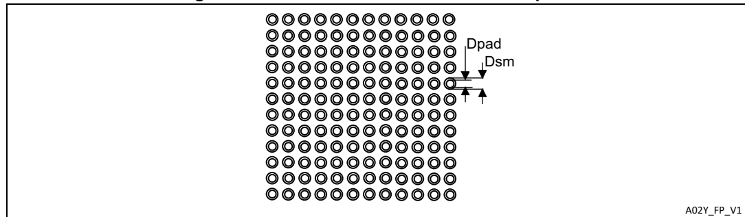
Figure 76. UFBGA144 recommended footprint
