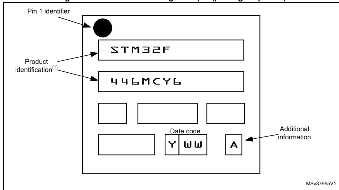
Figure 79. WLCSP81 marking example (package top view)
