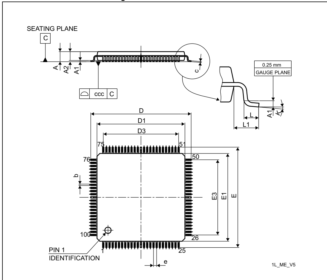
Figure 69. LQFP100 outline
