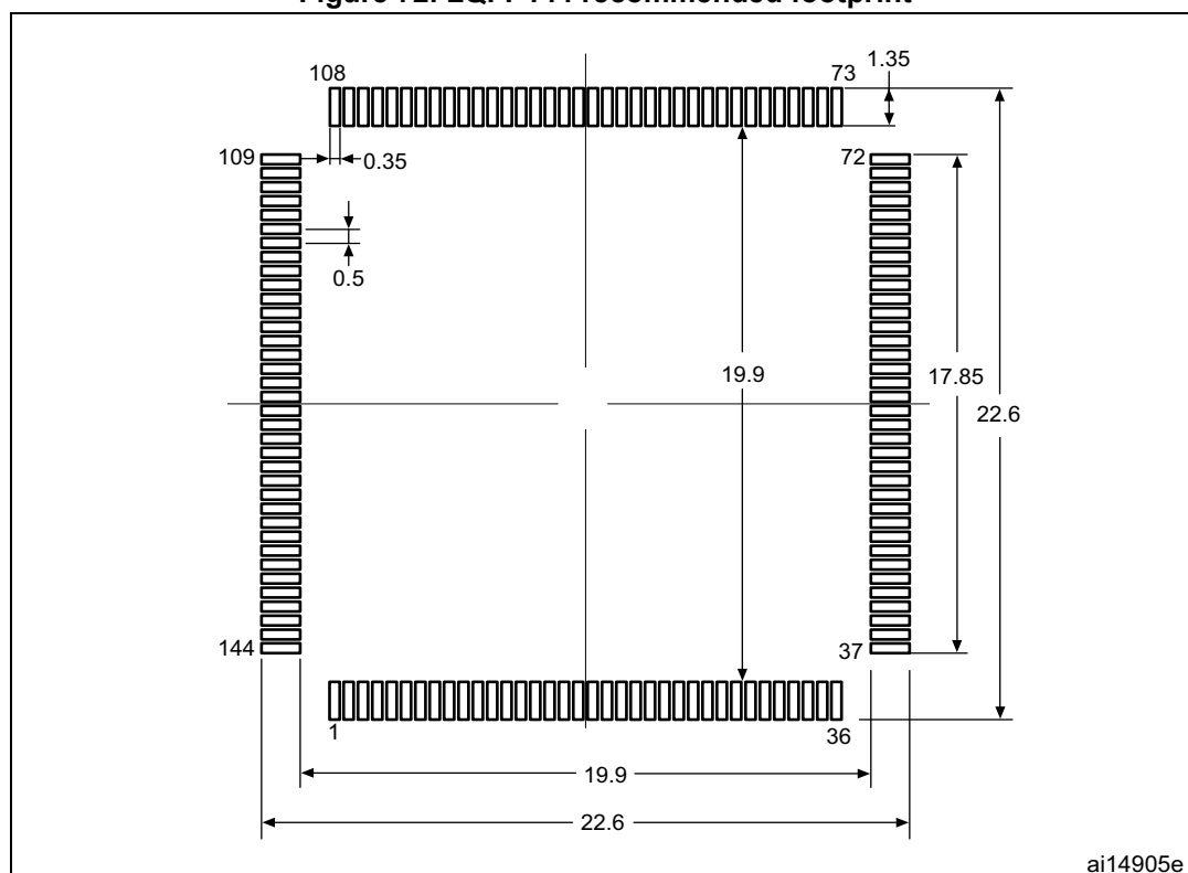
Figure 72. LQFP144 recommended footprint
