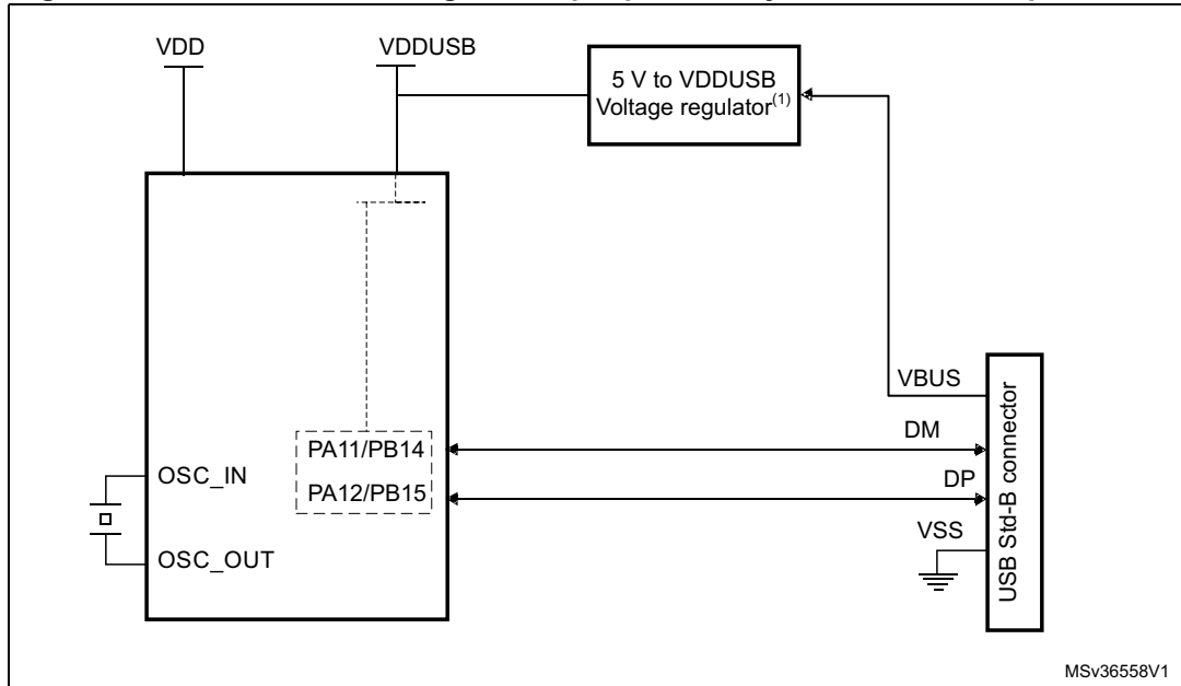
Figure 80. USB controller configured as peripheral-only and used in full speed mode
