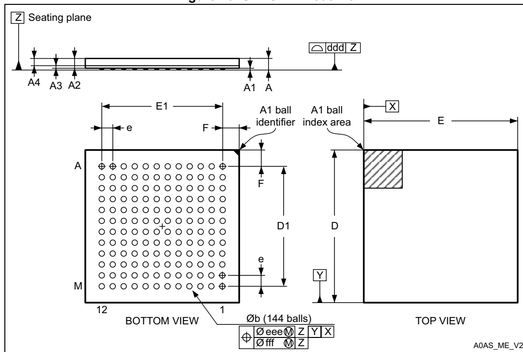
Figure 73. UFBGA144 outline
