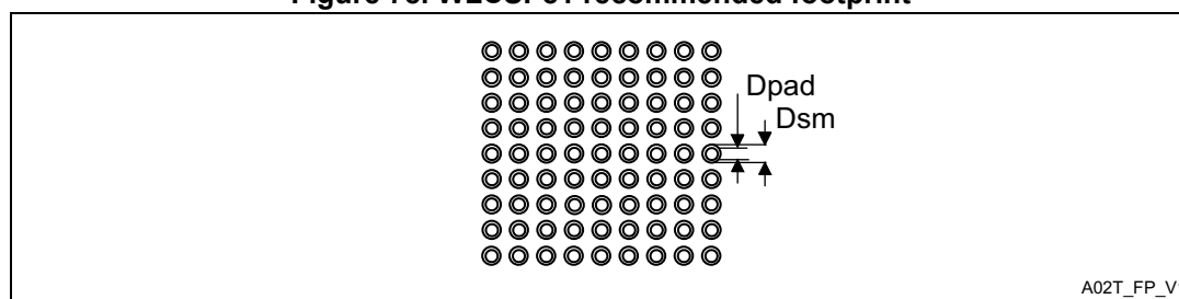
Figure 78. WLCSP81 recommended footprint
