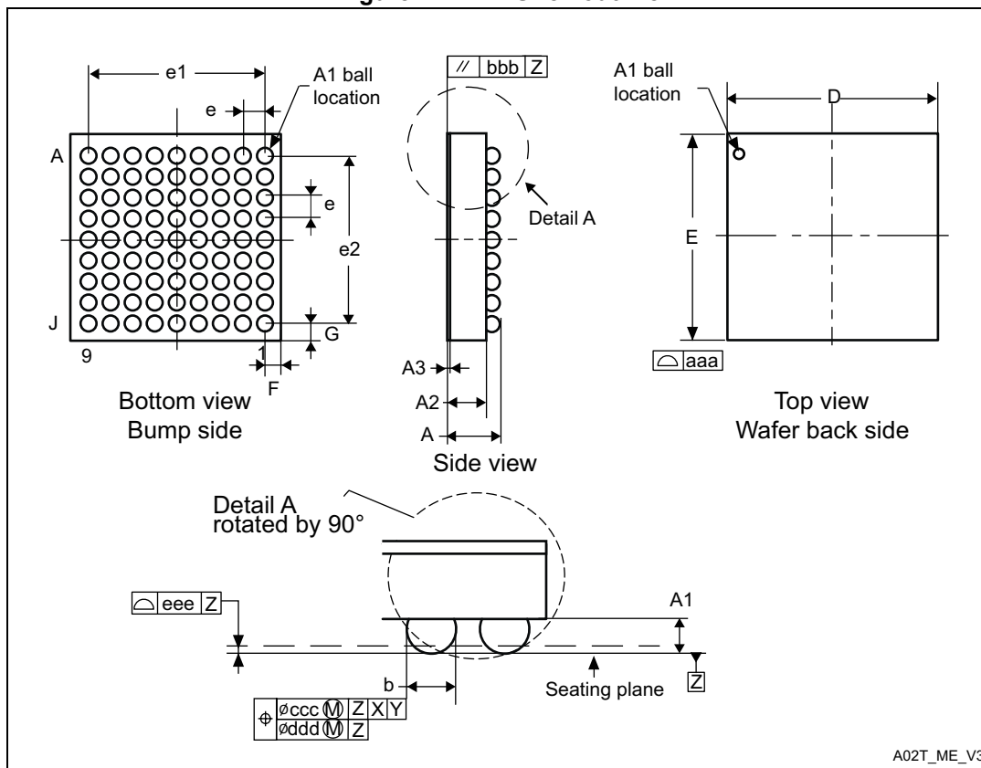
Figure 77. WLCSP81 outline
