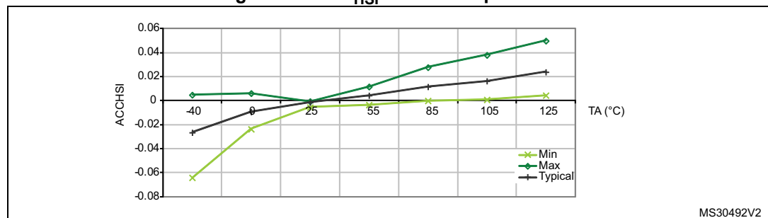
Figure 27. ACC_{HSI} versus temperature
