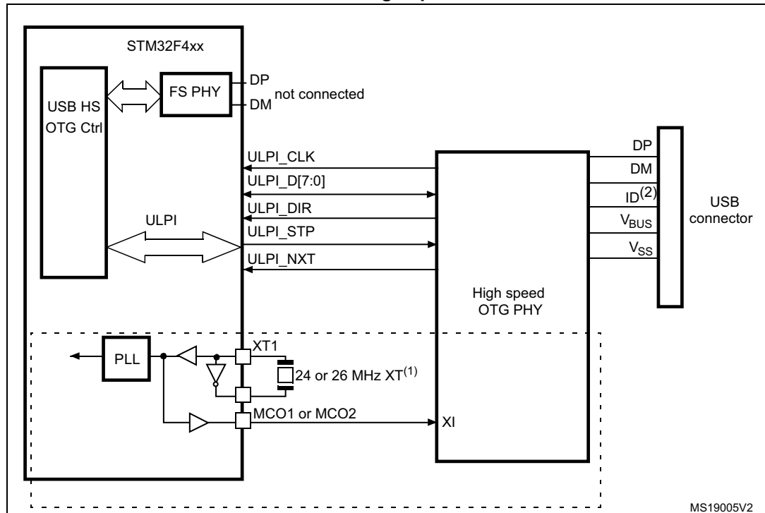
Figure 83. USB controller configured as peripheral, host, or dual-mode and used in high speed mode
