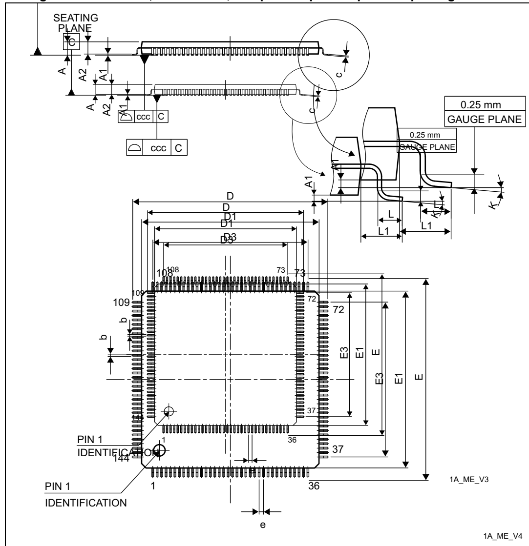
Figure 71. LQFP144, 20 x 20 mm, 144-pin low-profile quad flat package outline
