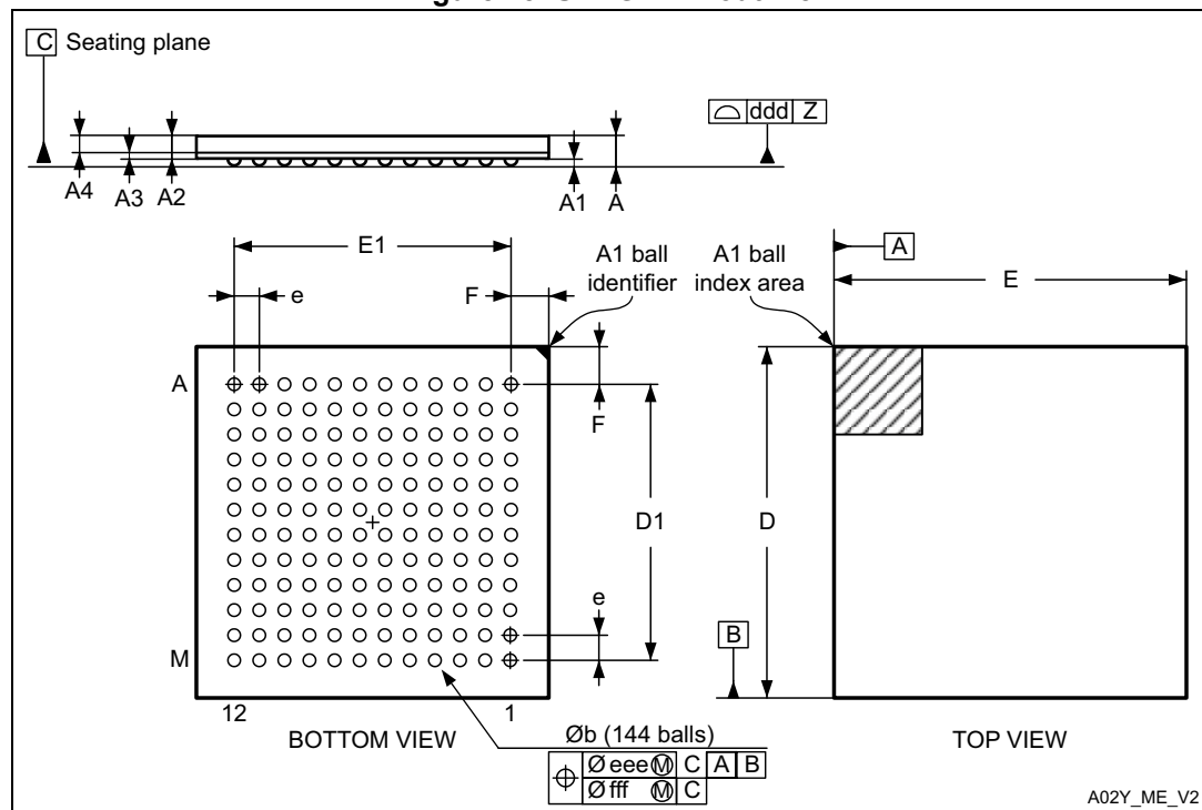
Figure 75. UFBGA144 outline
