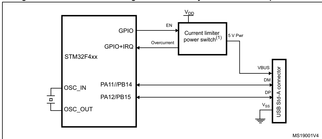
Figure 81. USB controller configured as host-only and used in full speed mode
