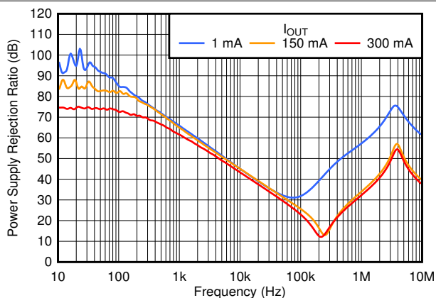
Figure 6-14. PSRR vs Frequency and I_{OUT}
