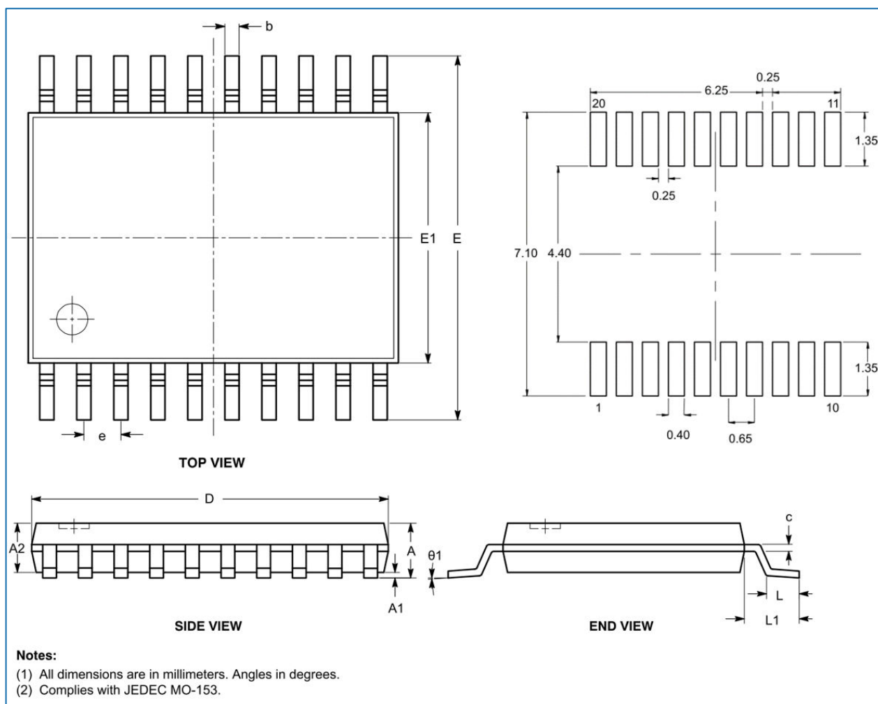
Figure 7-3 TSSOP20 package outline
