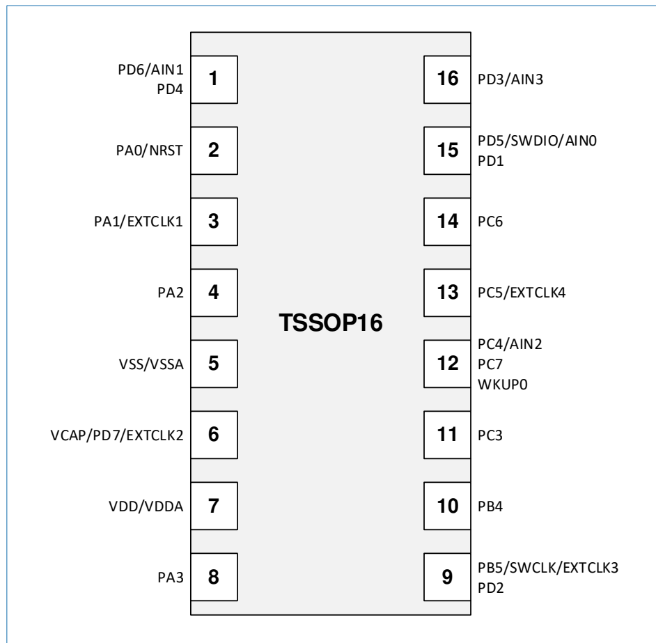
Figure 6-2 TSSOP16 (HK32F030MD4P6) package pinout
