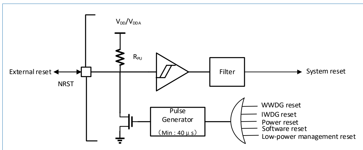
Figure 3-3 System reset
