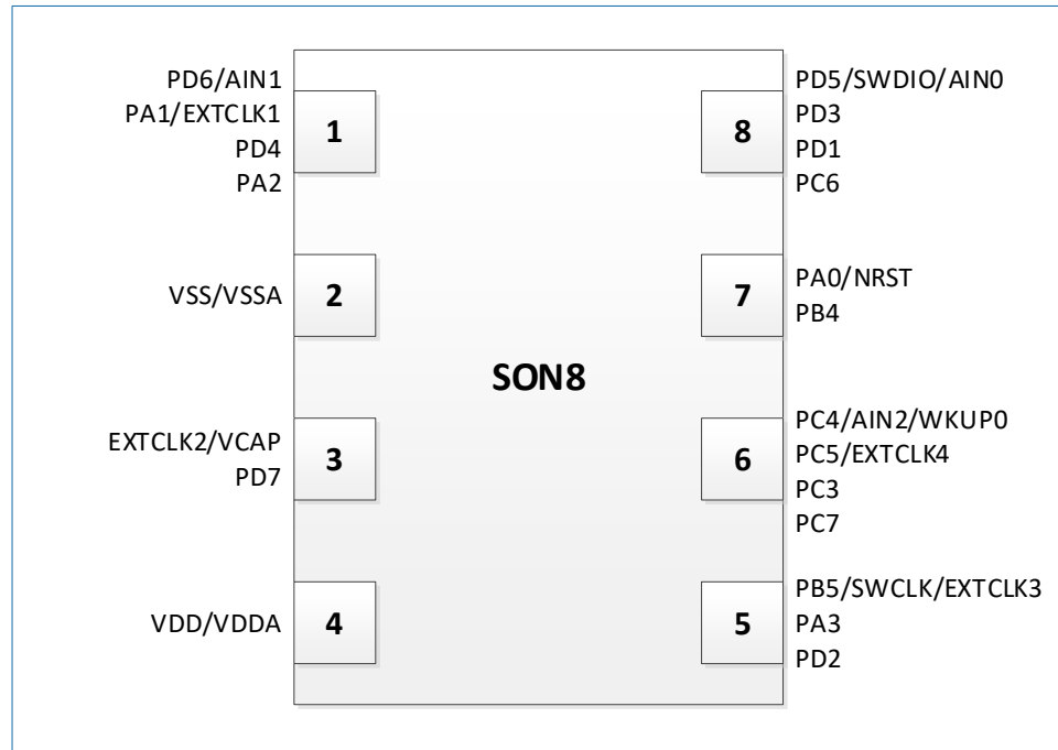
Figure 6-1 SON8 (HK32F030MJ4M6) package pinout
