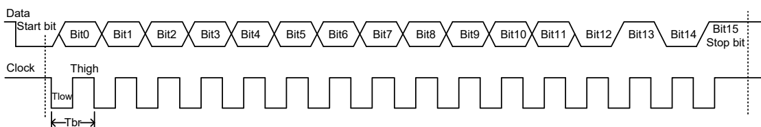
Data Transfer Timing – BS818C-2
