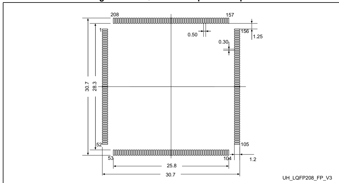
Figure 127. LQFP208 - footprint example
