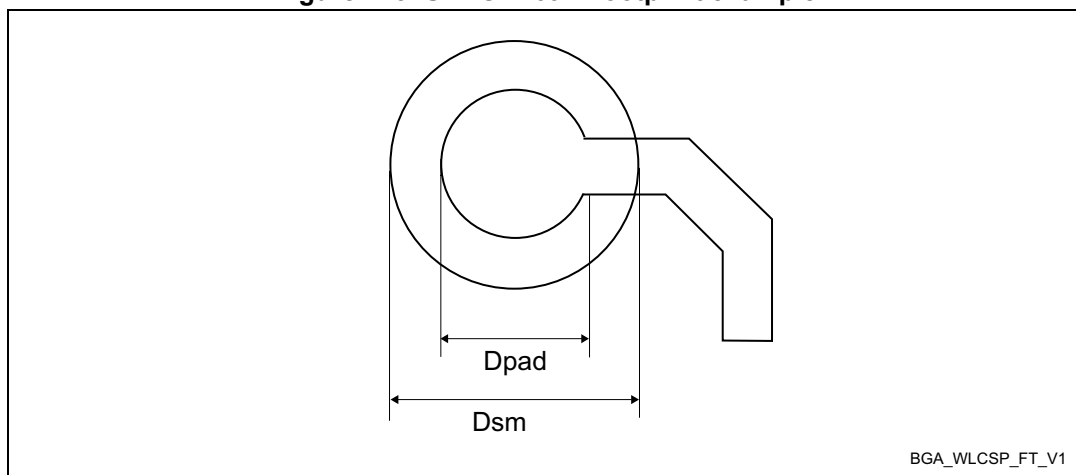
Figure 123. UFBGA169 - Footprint example
