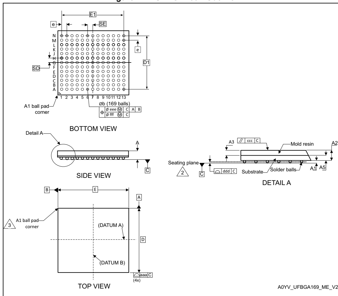
Figure 122. UFBGA169 - Outline
