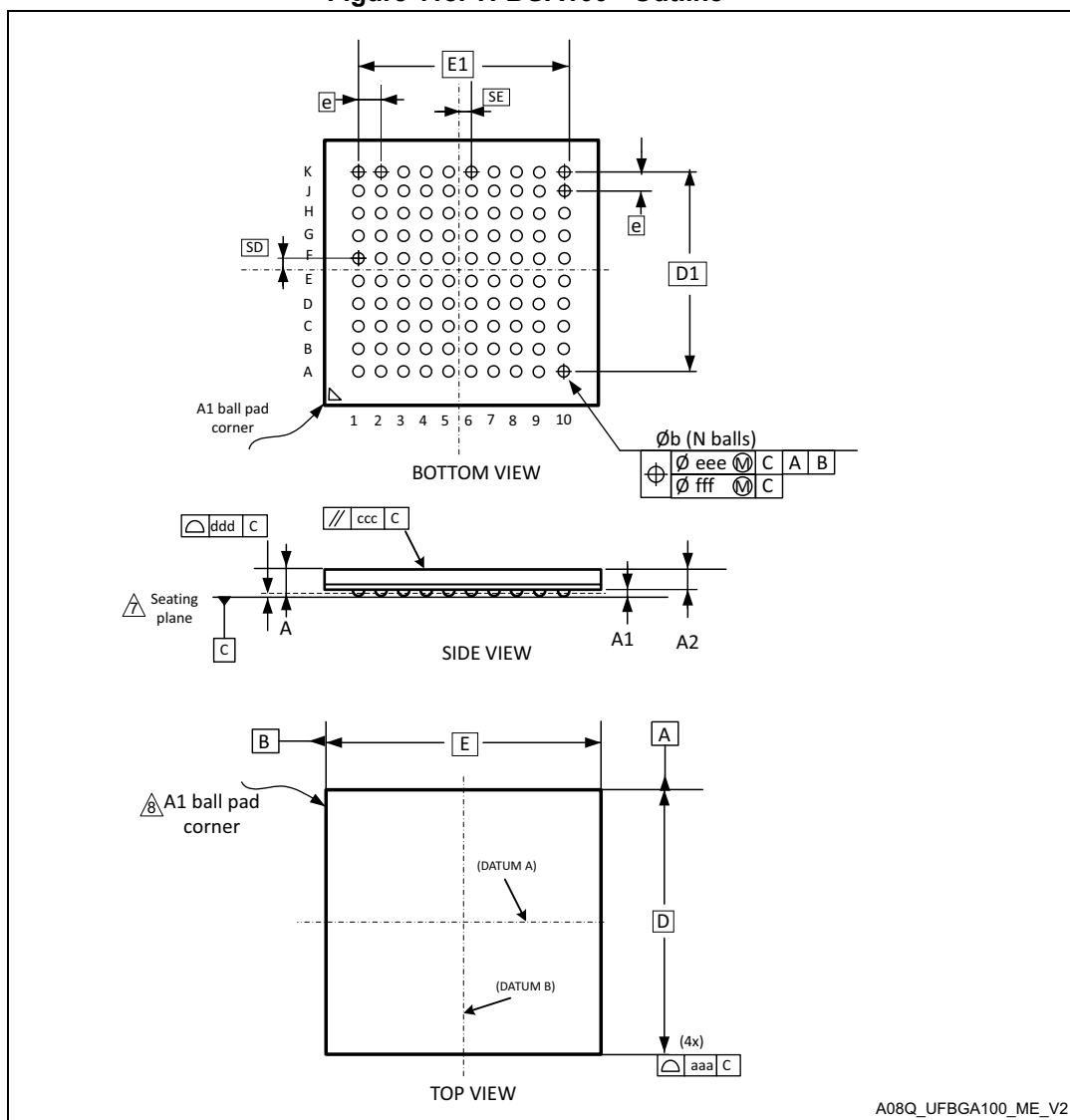
Figure 118. TFBGA100 - Outline (13)
