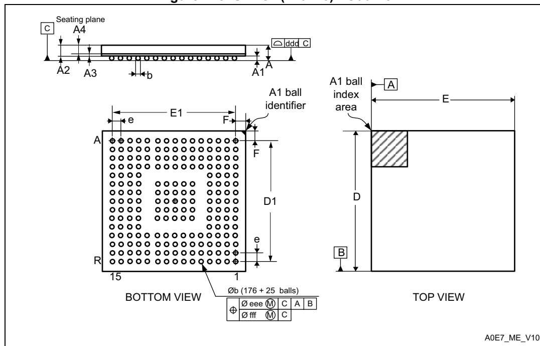
Figure 128. UFBGA(176+25) - Outline
