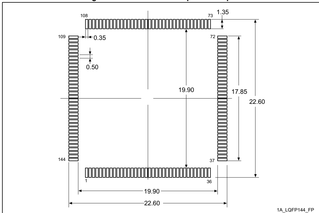
Figure 121. LQFP144 - Footprint example
