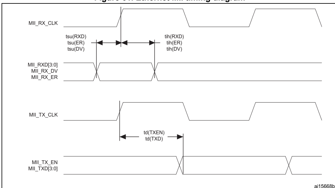
Figure 61. Ethernet MII timing diagram
