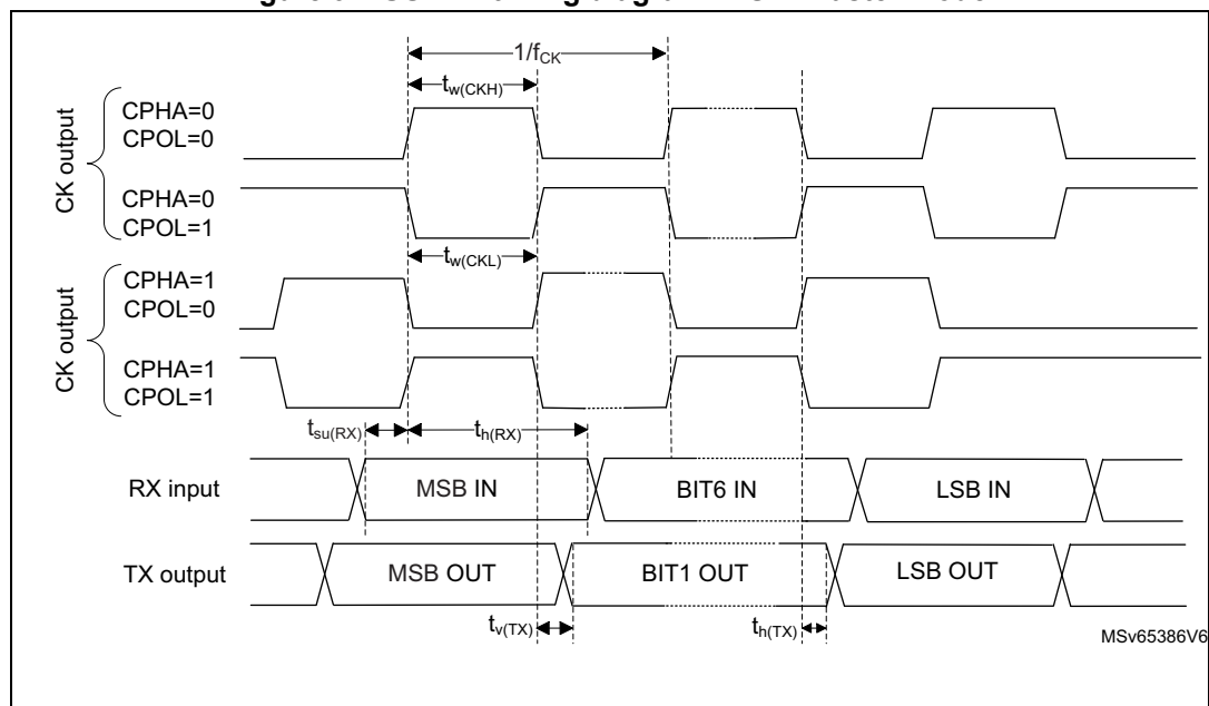
Figure 97. USART timing diagram in SPI master mode
