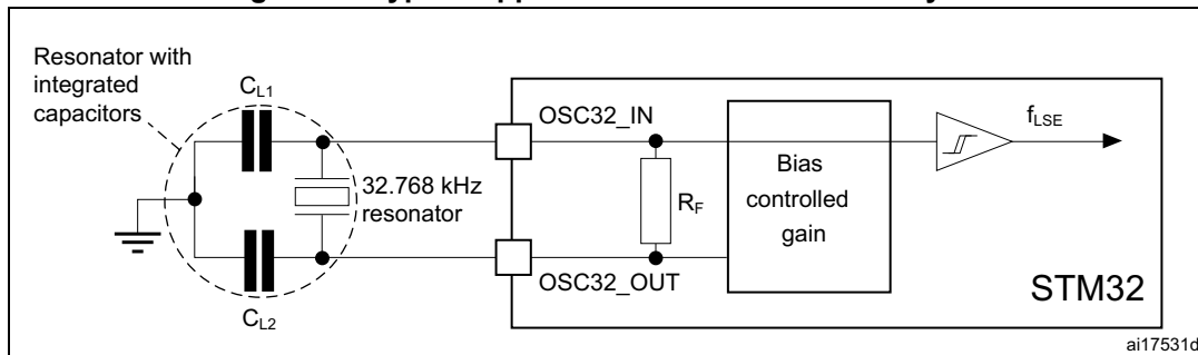
Figure 72. Typical application with a 32.768 kHz crystal
