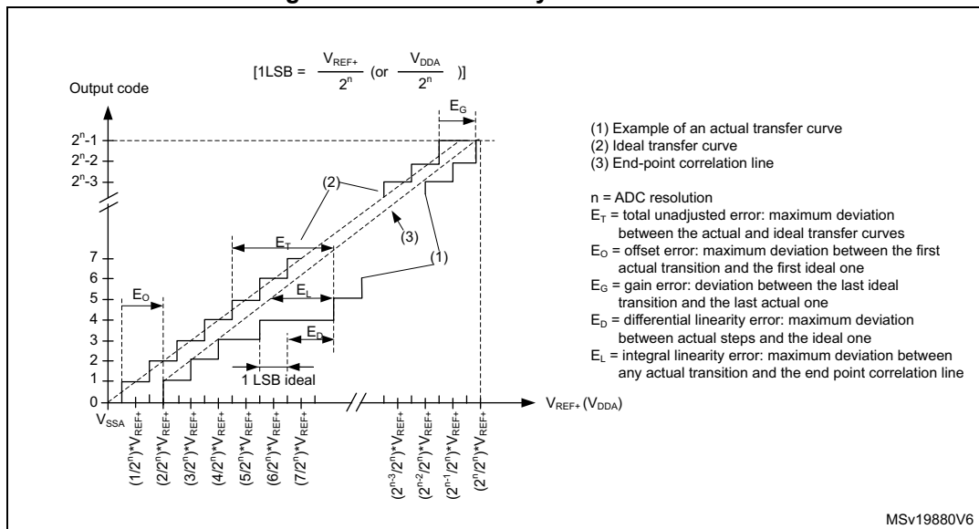
Figure 38. ADC accuracy characteristics
