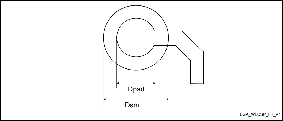
Figure 119. TFBGA100 - Footprint example
