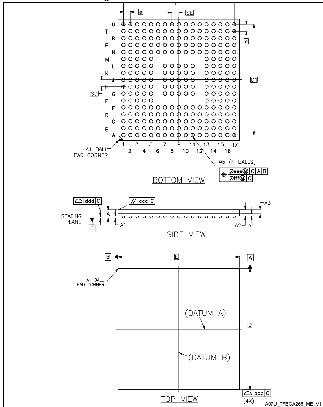
Figure 130. TFBGA240+25 - Outline
