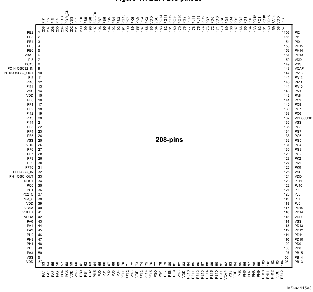
Figure 11. LQFP208 pinout
