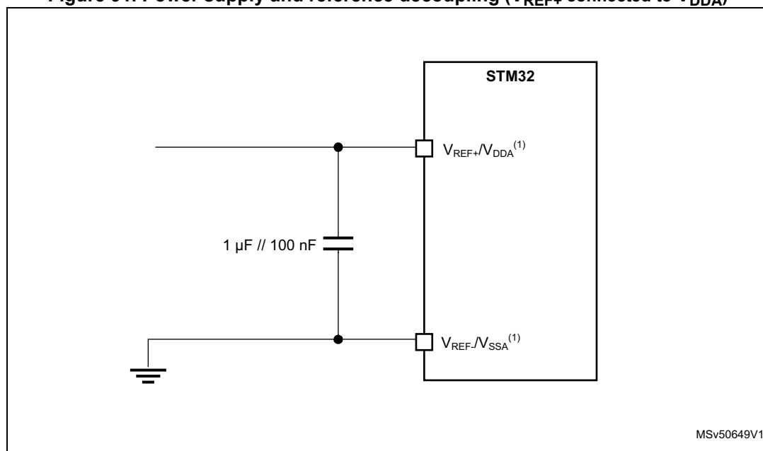
Figure 91. Power supply and reference decoupling ( V_{REF+} connected to V_{DDA} )
