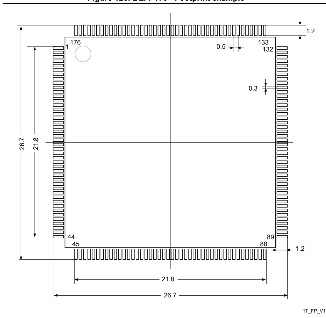
Figure 125. LQFP176 - Footprint example
