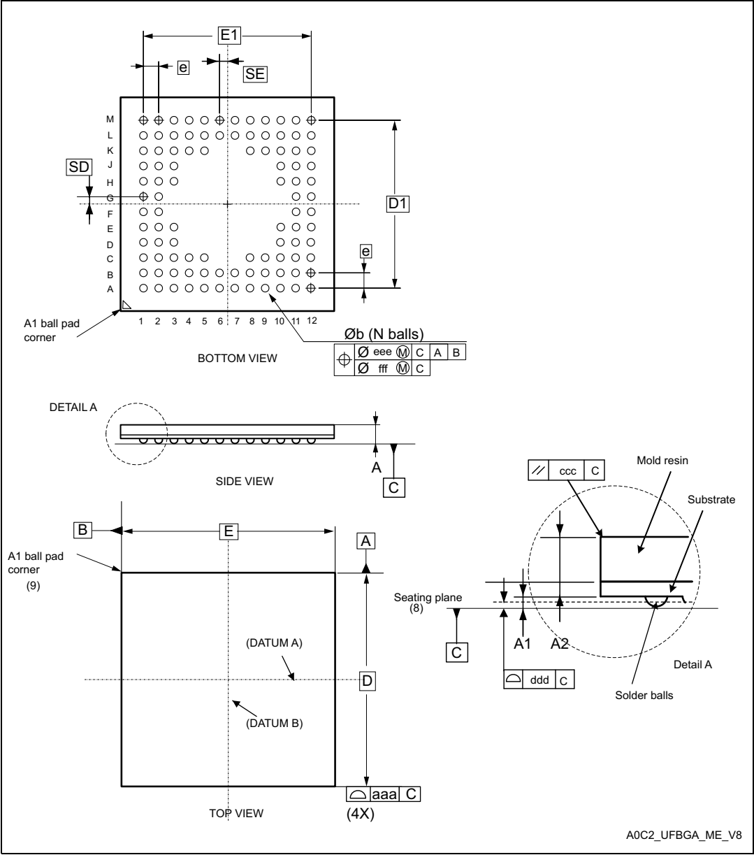
Figure 54. UFBGA100 - Outline (13)
