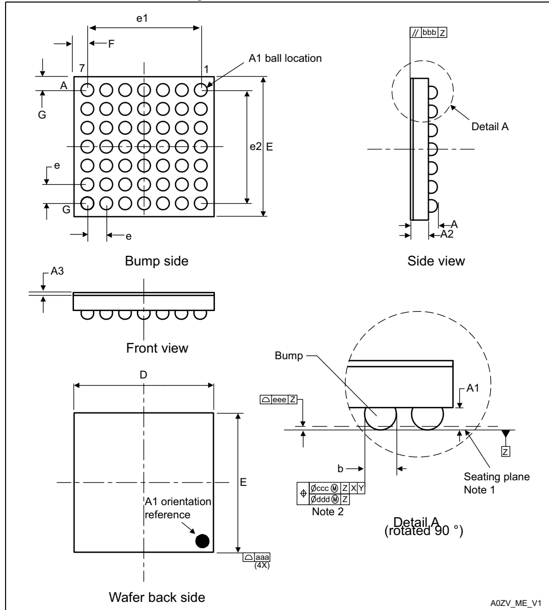
Figure 46. WLCSP49 - Outline
